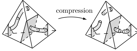
Figure 6: A compression in the interior of a cell. This move reduces the local Euler number and does not change weight or the 0-weight curves in the interior of faces of \mathcal{T} .
